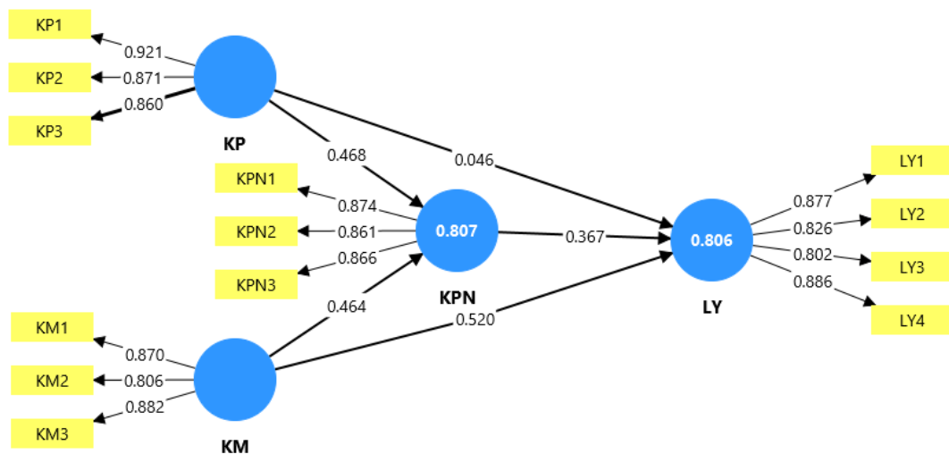
Gambar 4.1: Outer Model 1
